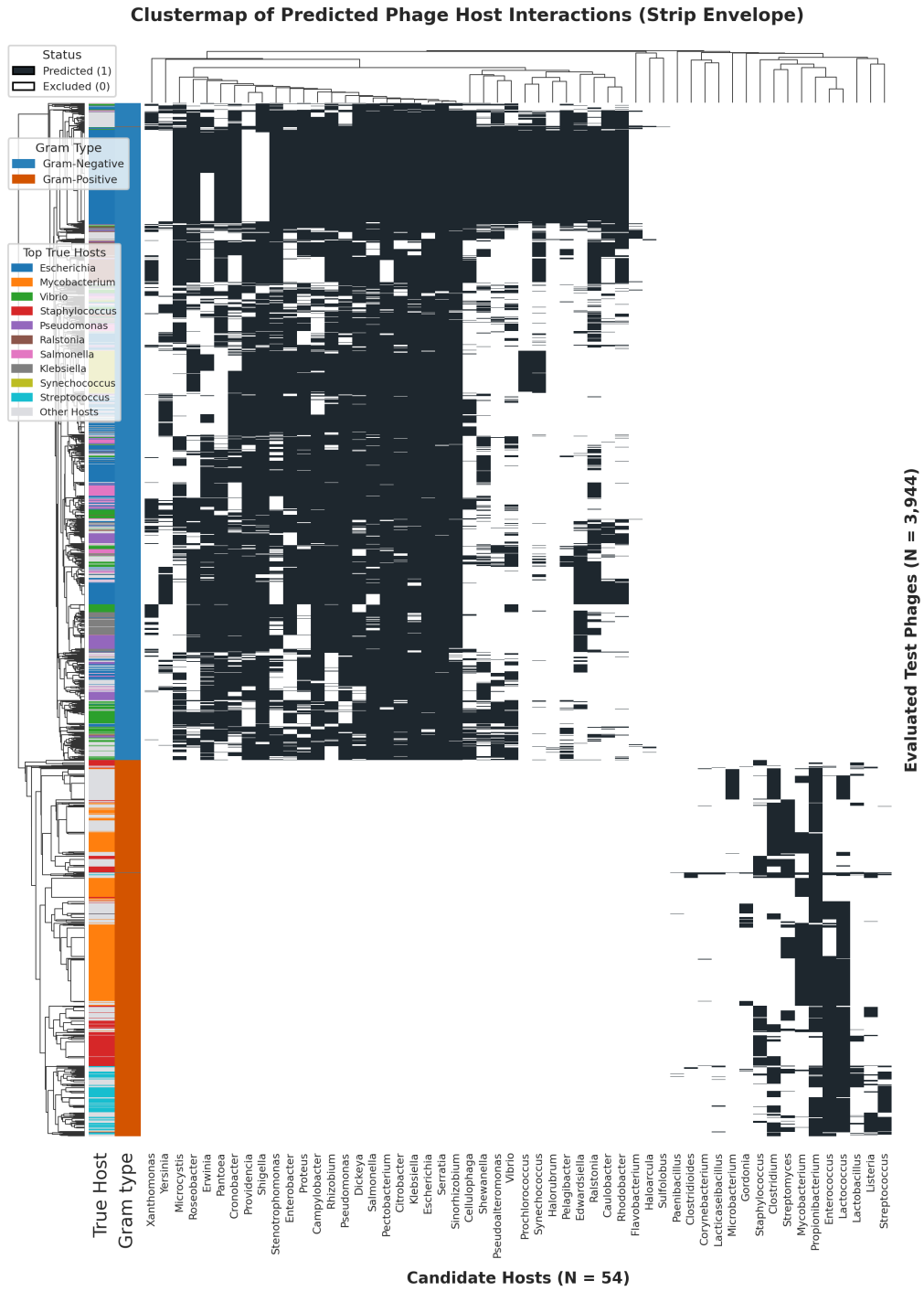
Figure A.11: Clustermap of Predicted Phage Host Interactions (Strip Envelope). Binary prediction matrix across N_{\text{test}} = 3,944 test phages and 54 host genera for the Strip envelope ( N_B = 10, w = 2 ).
