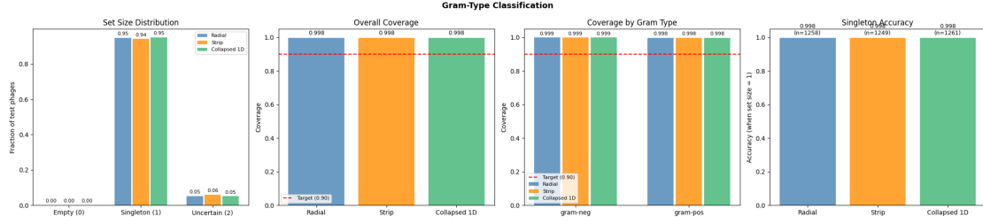
Figure 5.1: Gram type classification performance across Radial, Strip, and Collapsed 1D geometries on the test split (Fold 0, nominal target 1 - \alpha = 0.90 ). Panels show (left to right): prediction set size distribution, marginal empirical coverage, class-conditional coverage, and singleton accuracy with sample counts ( n ).
