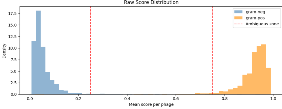
Figure 5.2: Distribution of raw scores per test phage, separated by true Gram type. Gram negative phages concentrate tightly near 0 while Gram positive phages concentrate near 1, leaving the intermediate ambiguous zone (0.25–0.75, dashed red lines) almost empty.
