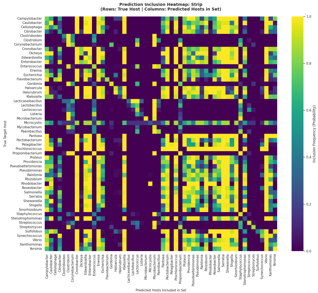
Figure A.9: Prediction set inclusion frequency heatmap for the Strip envelope across all 54 true hosts (rows) vs. predicted candidate hosts (columns).
